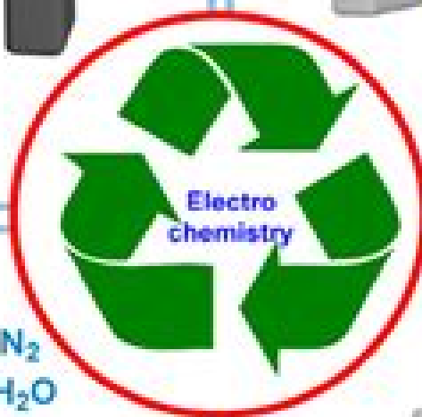
Electrophotocatalysis
