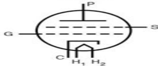
Tetrode
