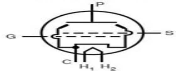
Beam tetrode
