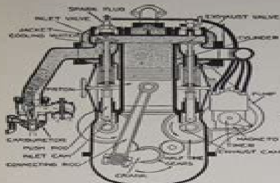
SUCTION STROKE
