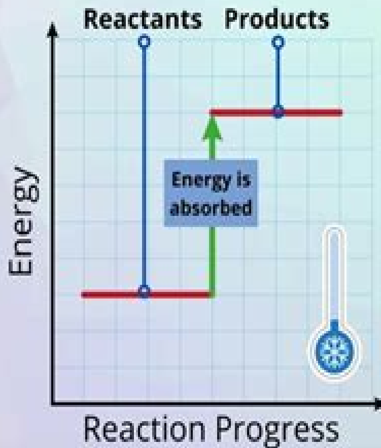
Endothermic Reaction
