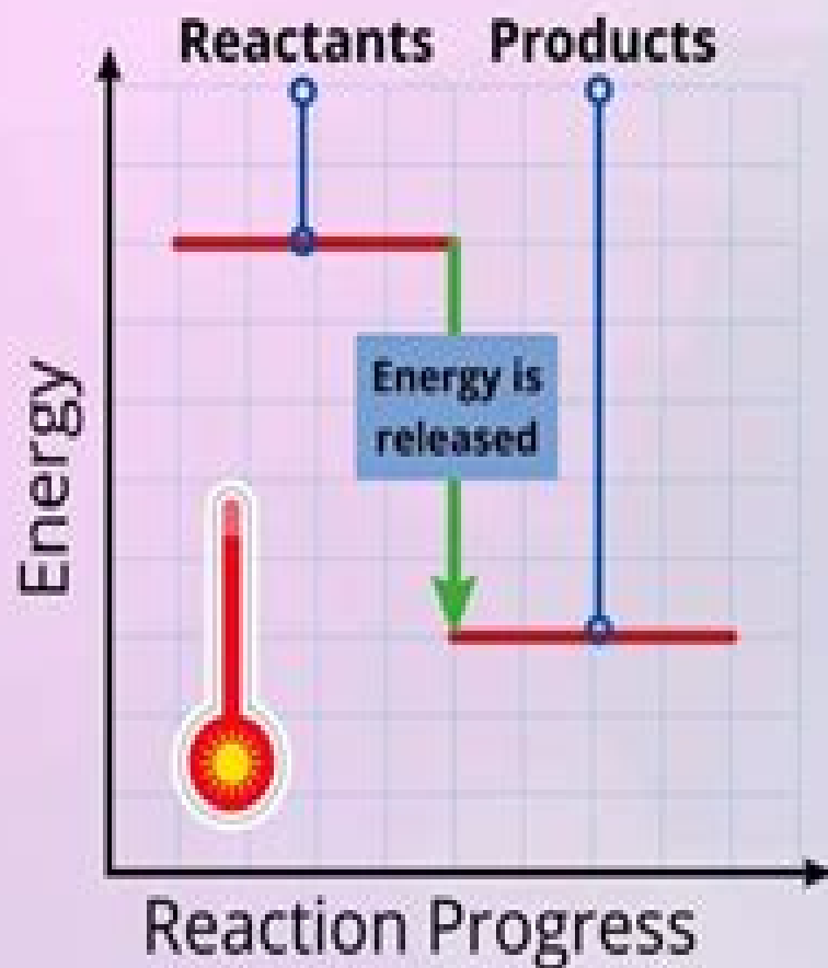
Exothermic Reaction
