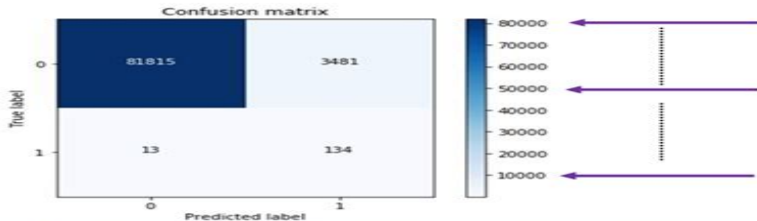
(c) Confusion Matrix for Whole Data Set
