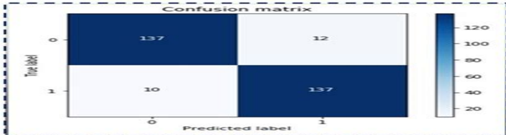
(b) Confusion Matrix for Test Data Set
