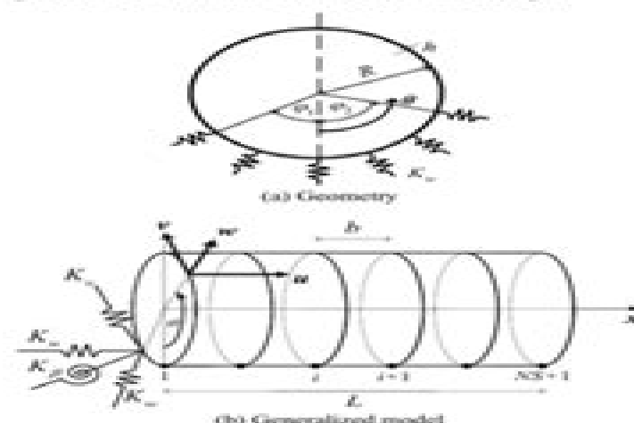
Fig.1. Cylindrical shell on elastic foundation.
