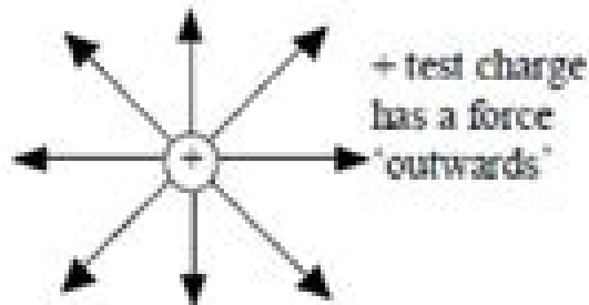
Positive point charge
