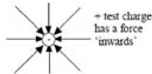
Negative point charge
