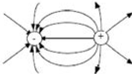
Positive and negative point charges
