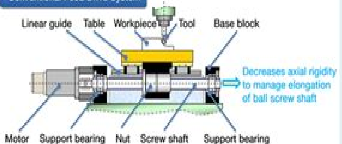
Conventional Feed Drive System
