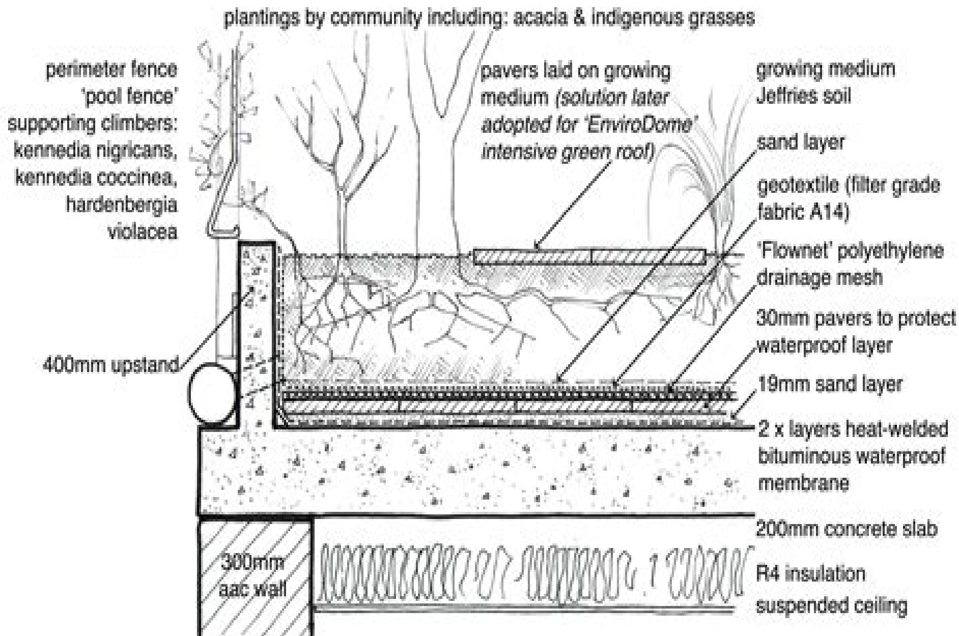
SECTION THROUGH INTENSIVE ROOF GARDEN
