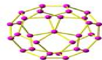
32 ( D_3 )
