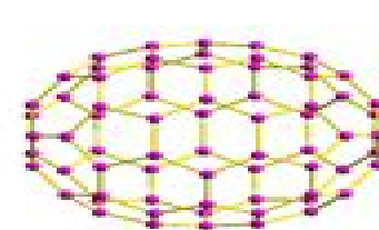
70 ( D_{5h} )
