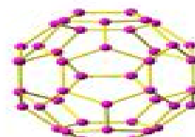
46 ( C_{2v} )
