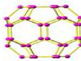
36 ( D_{6h} )
