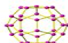
30 ( C_{2v} )
