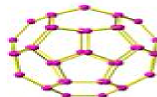
44 ( D_{3h} )
