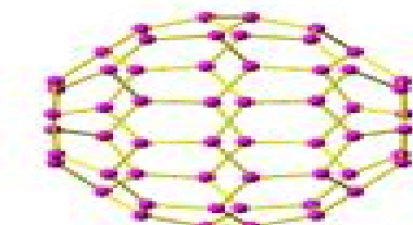
56 ( D_2 )
