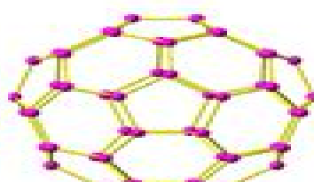
50 ( D_{5h} )
