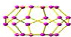
24 ( D_{6h} )
