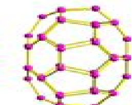
48 ( D_{6d} )
