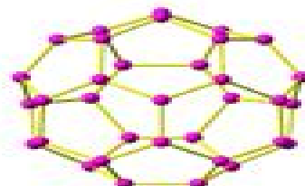
34 ( C_{3v} )
