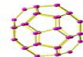
40 ( D_{5d} )
