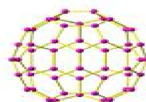
54 ( C_{2v} )
