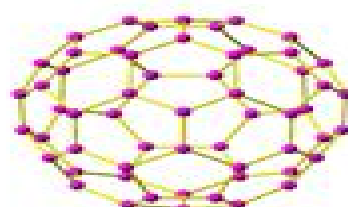
58 ( C_{3v} )
