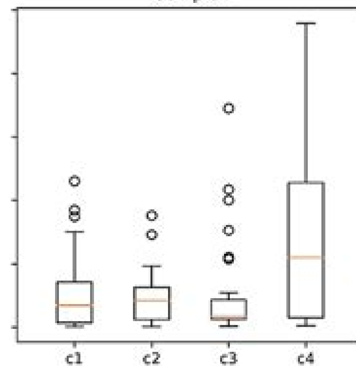
box plot
