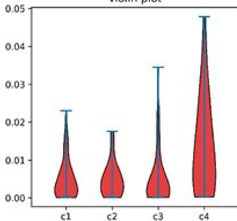
violin plot
