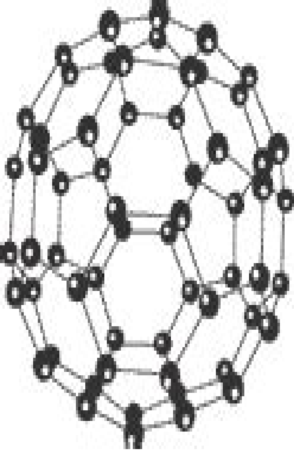
C 60 : prototype fullerene
