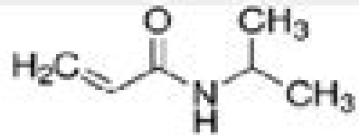
N-isopropylacrylamide (NIPAM)
