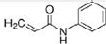
N-phenylacrylamide (PAM)
