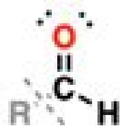
aldehyde
