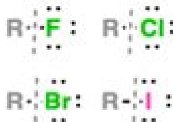
alkyl halide
