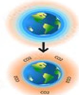
Greenhouse Effect
