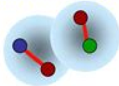
Hadronic molecule
