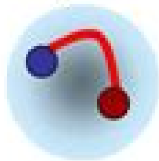
Hybrid
