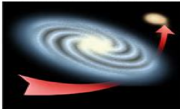
1. Disk galaxy and companion.
