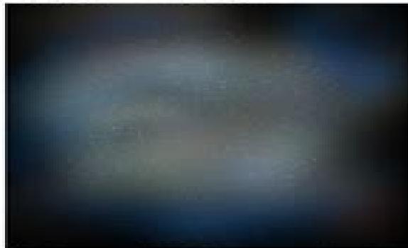
1. Primordial hydrogen cloud.
