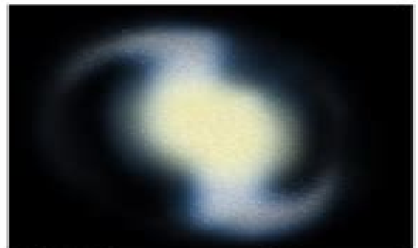
3. As bulge grows with new stars the bar is disrupted and dissipates.
