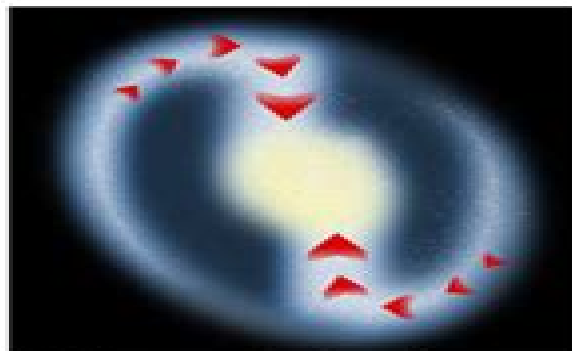
2. Disk perturbations form a bar-like structure which shovels fresh gas into the center.
