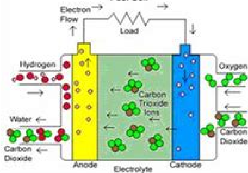
Molten Carbonate Fuel Cell
