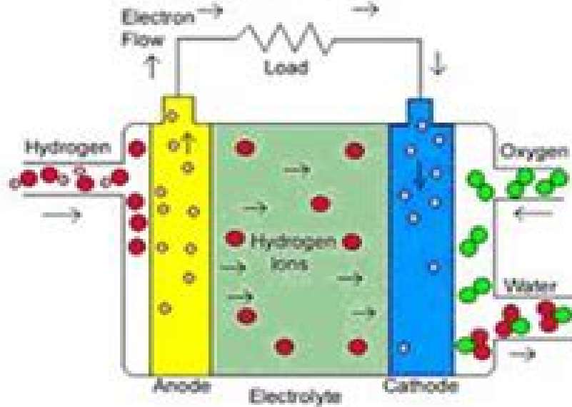
Phosphoric Acid and P.E.M. Fuel Cells
