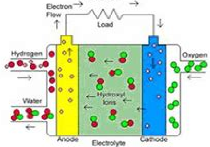
Alkali Fuel Cell
