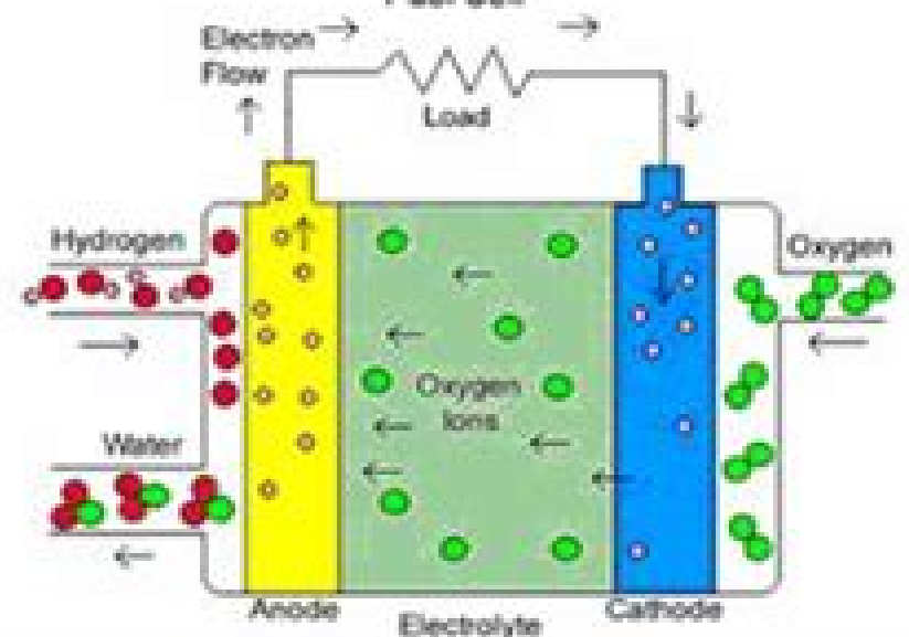
Solid Oxide Fuel Cell
