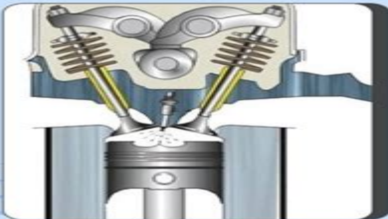
DIRECT INJECTION
