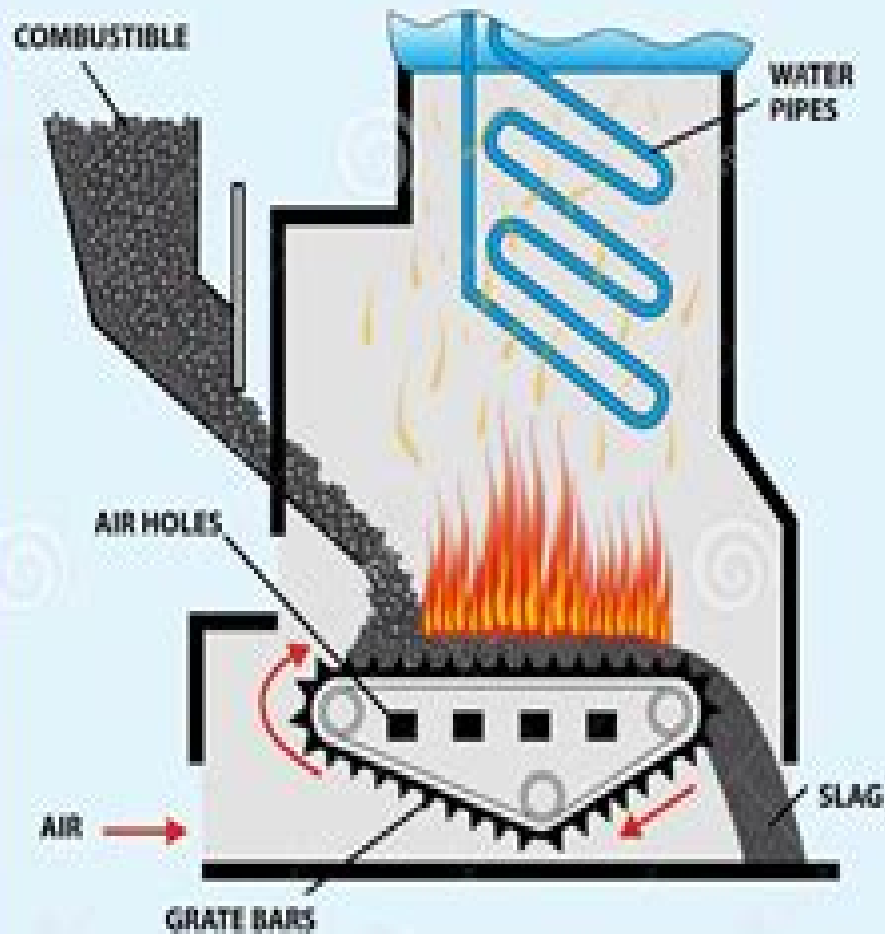
SOLID FUEL FURNACE
