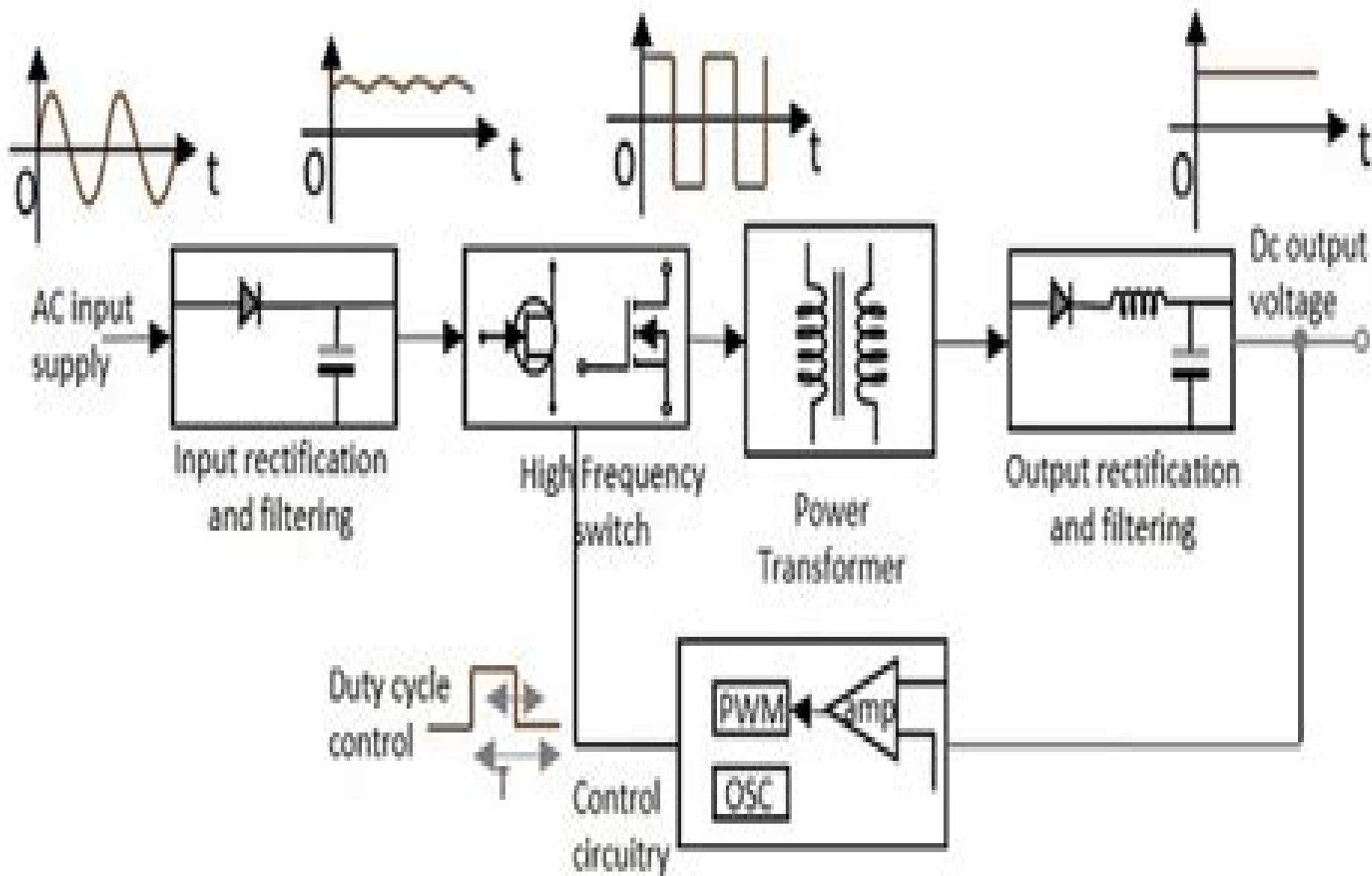
Functional block diagram of SMPS
