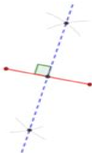
Perpendicular Bisector
