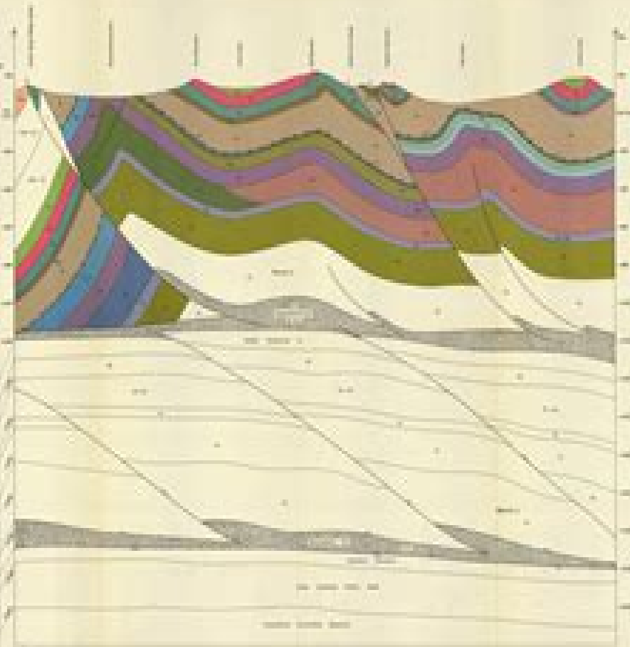
CROSS SECTION QUAD. LINE 5-5
