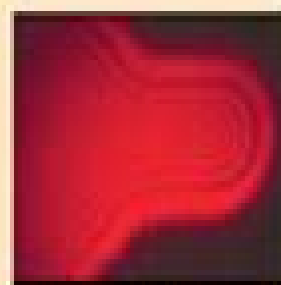
Barrier Diffraction
