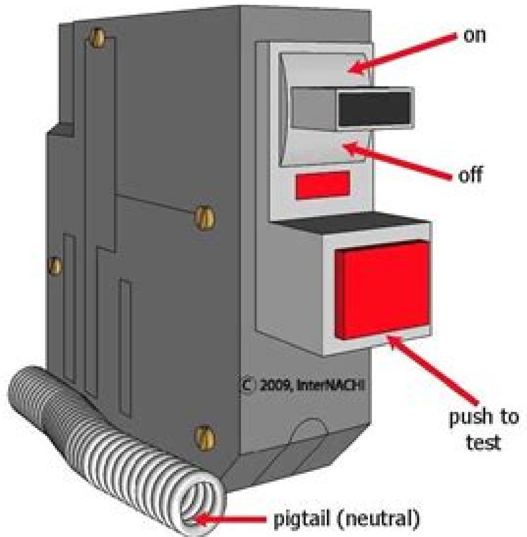
CIRCUIT BREAKER
