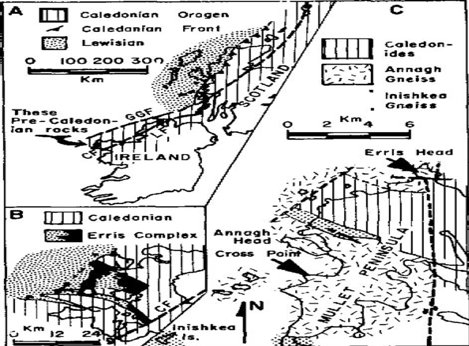
FIG. 1. Location and general geological map of the
