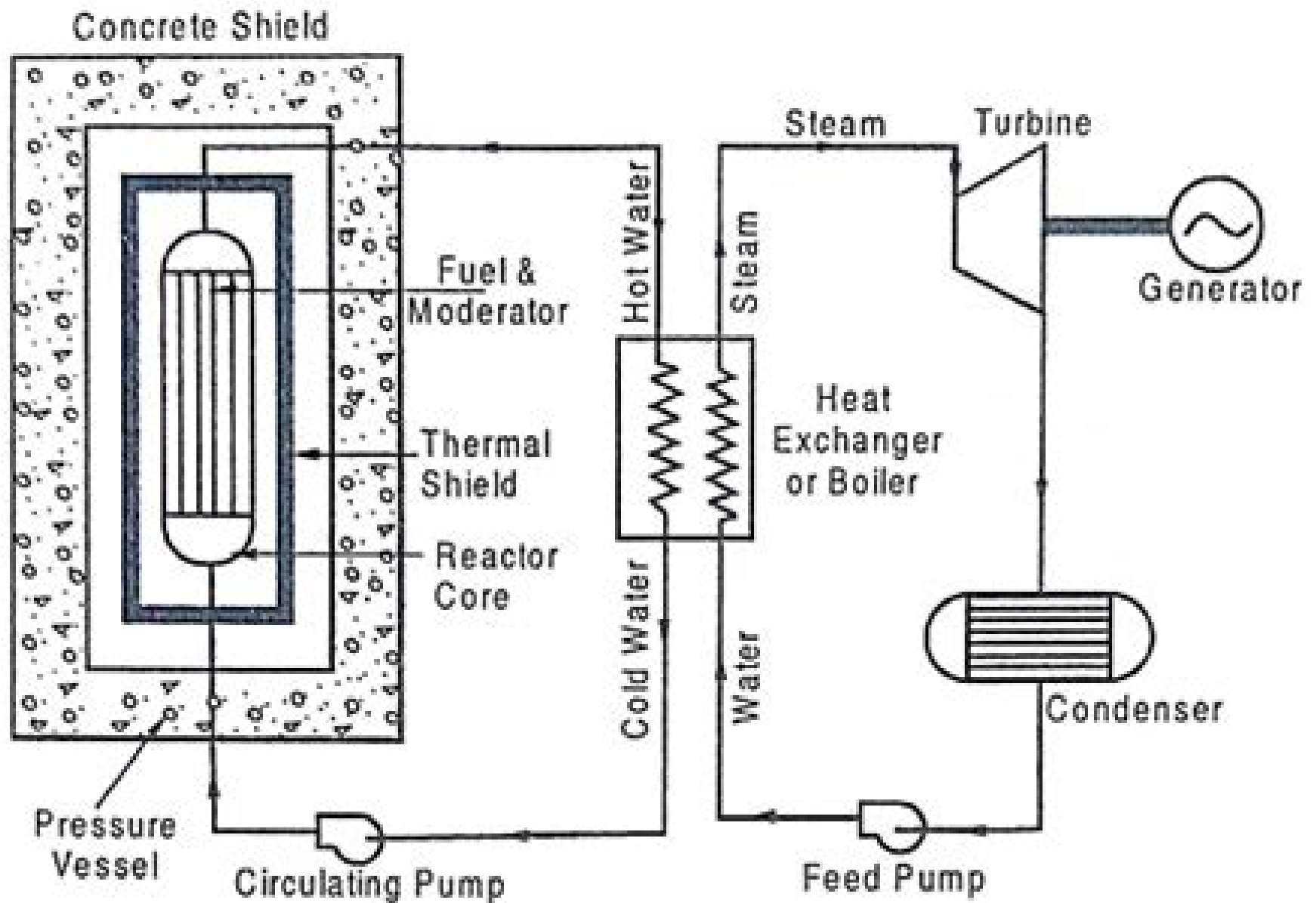
Fig:3.4 Layout of Nuclear Power Plant
