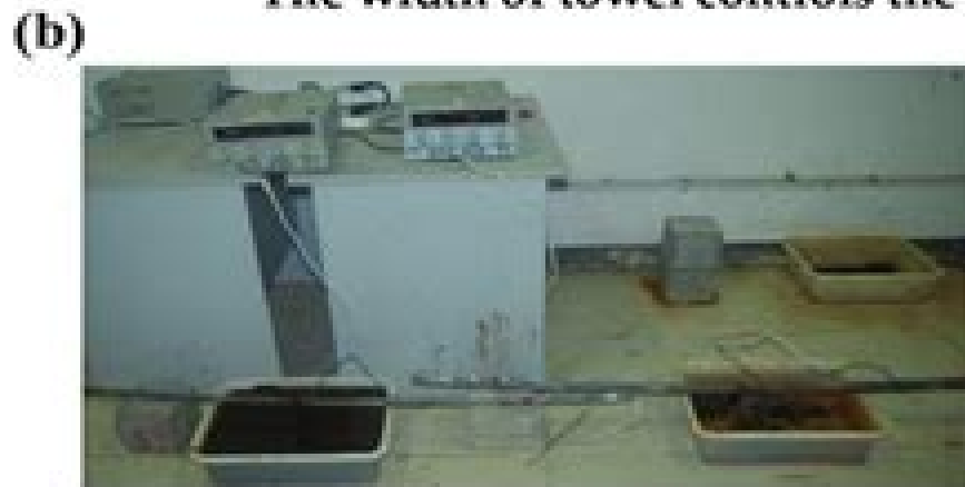
The electrochemical accelerated corrosion of P1 and P2 in situ
