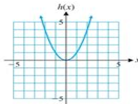
(B) Square function h(x) = x^2 Domain: R Range: [0, \infty)
