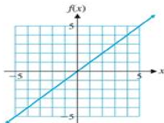
(A) Identity function f(x) = x Domain: R Range: R
