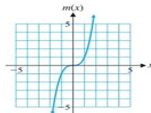
(C) Cube function m(x) = x^3 Domain: R Range: R
