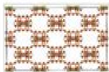
Attapulgite
