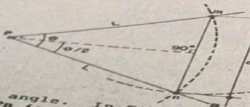
Fig. 11-4. Laying off an angle using a chord length.
