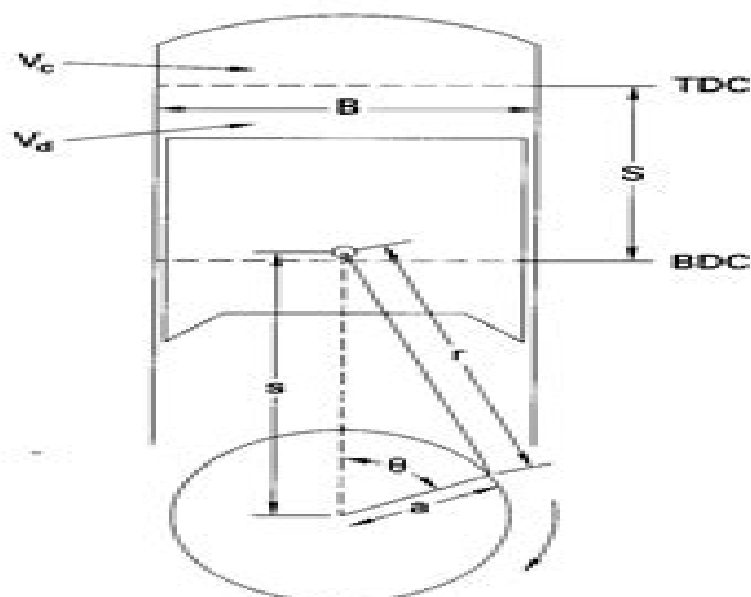
Figure 2-1 Piston and cylinder geometry of reciprocating engine. B = bore; S = stroke; r = connecting rod length; a = crank offset; s = piston position; \theta = crank angle; V_c = clearance volume; V_d = displacement volume.
