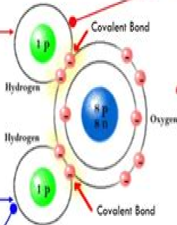
Bohr Model of H 2 O
