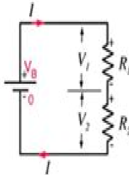
Series resistors
