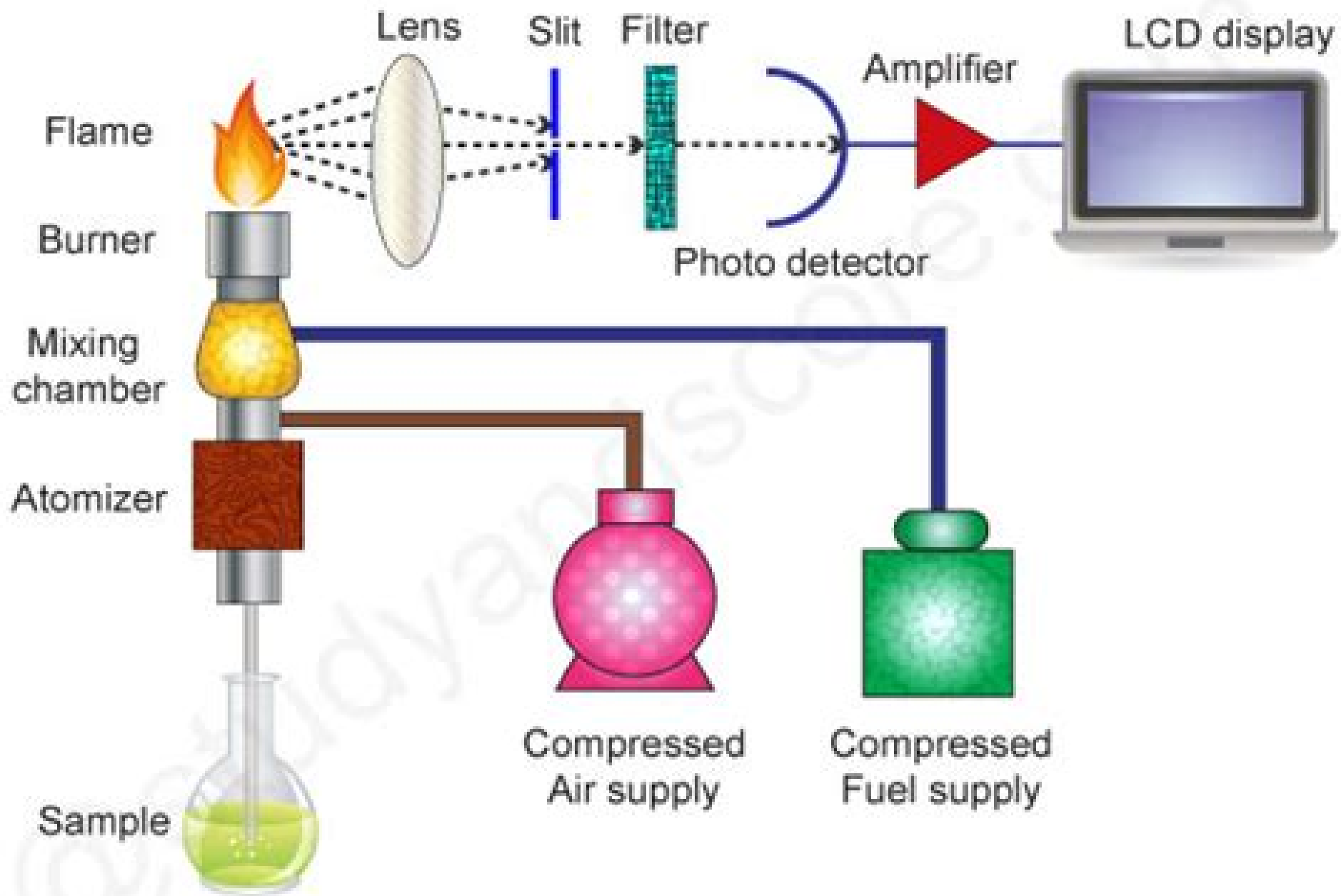
FLAME PHOTOMETER
