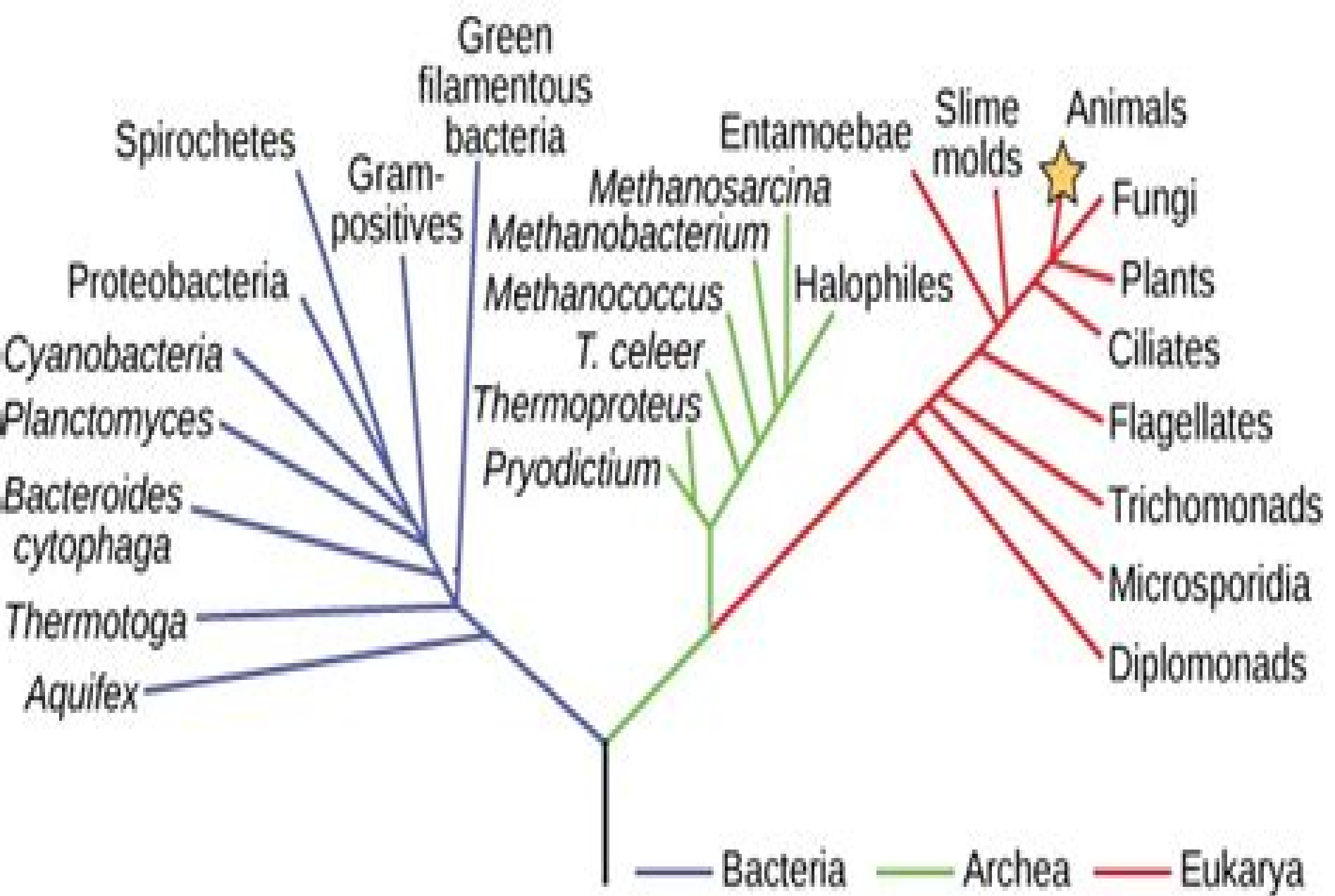
(a) Rooted phylogenetic tree
