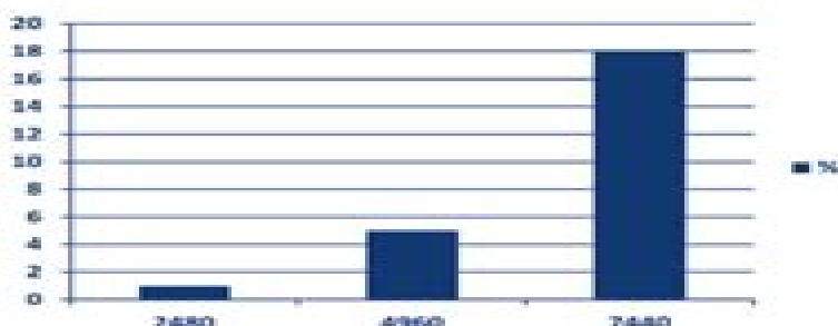
Fig. 1. Percent under-size channel catfish harvested from single batch production ponds stocked at three densities ranging from 2480 to 7440 fish per hectare (adapted from Engle, 2010).*
