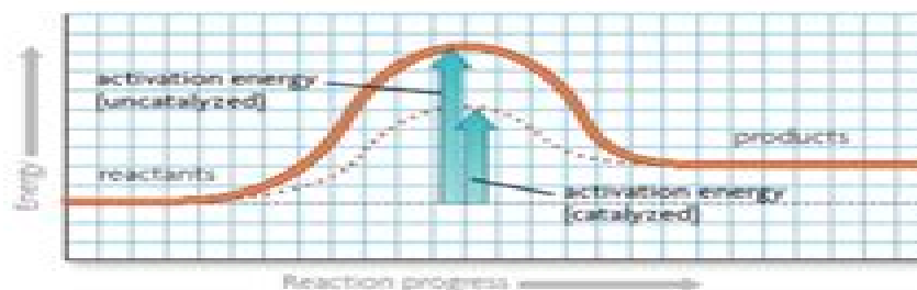
FIGURE 5.1 CATALYSTS AND ACTIVATION ENERGY
