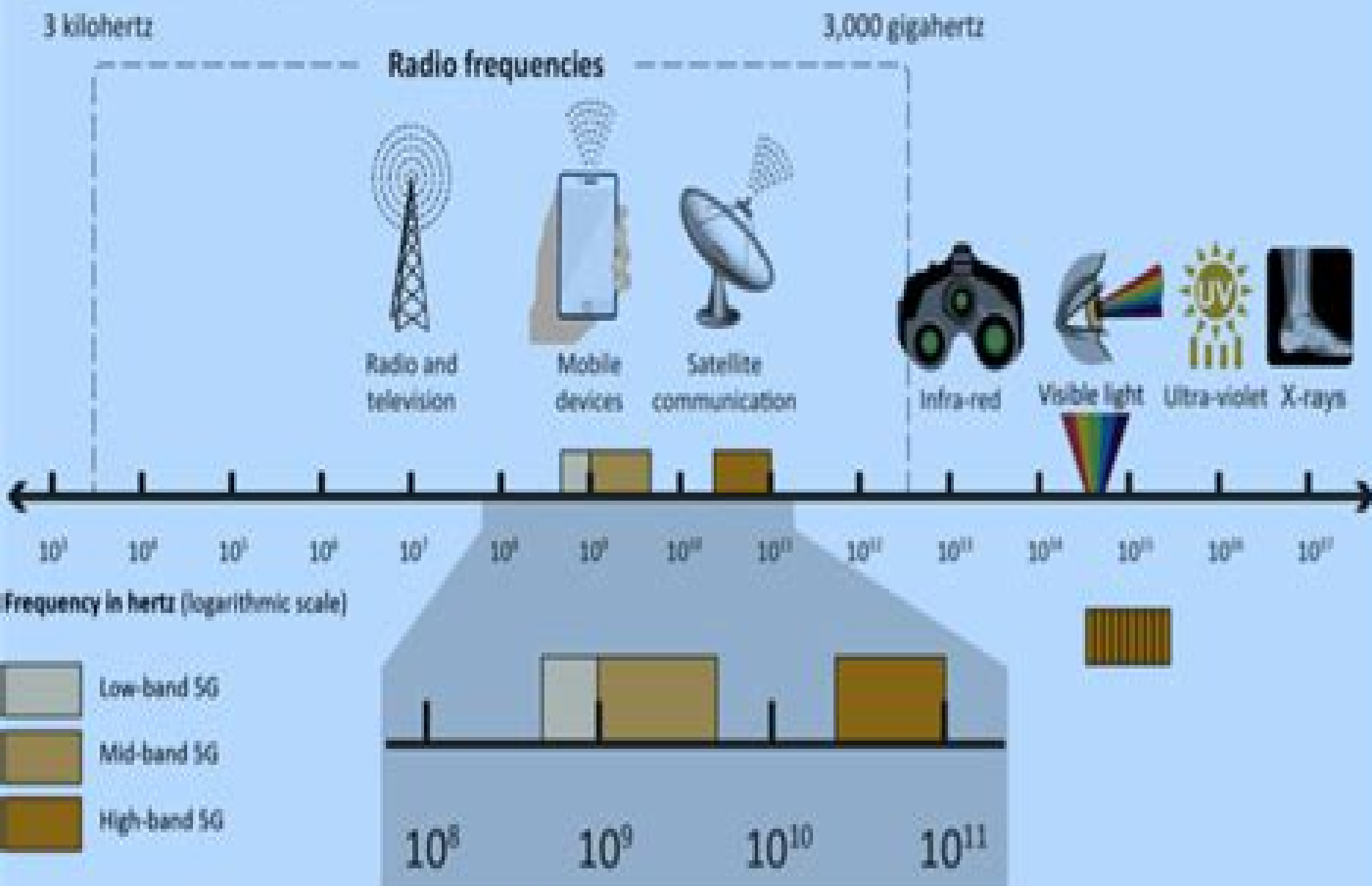
Figure 2: Electromagnetic spectrum
