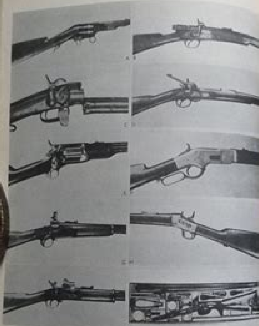
Plate 19. A. Colt "Patented" Ring Lever revolving rifle, Second Model. (G.M.A.G.) B. Collier & Terry Capping Carbine. (R.M.) C. Grant Carbine made by Mann, Arm Co., U.S.A., with Mowat's Tap Primer. Action open. (G.M.A.G.) D. Wadley-Richards "Wadley-Tail" Carbine. Action open. (G.M.A.G.) E. Colt '56 caliber revolving carbine. (G.M.A.G.) F. Henry '44 Boreless brass frame rifle. (G.M.A.G.) G. Soper rifle - 1840 caliber. Action open. (G.M.A.G.) H. Remington 11-43 mm. caliber Express Model (R.M.) I. Smith - 177 caliber rifle. Action open. (Author's Collection.) J. Case's Double Rifle one gauge rifling. 30 gauge, by John Dickson, Edinburgh. (G.M.A.G.)
