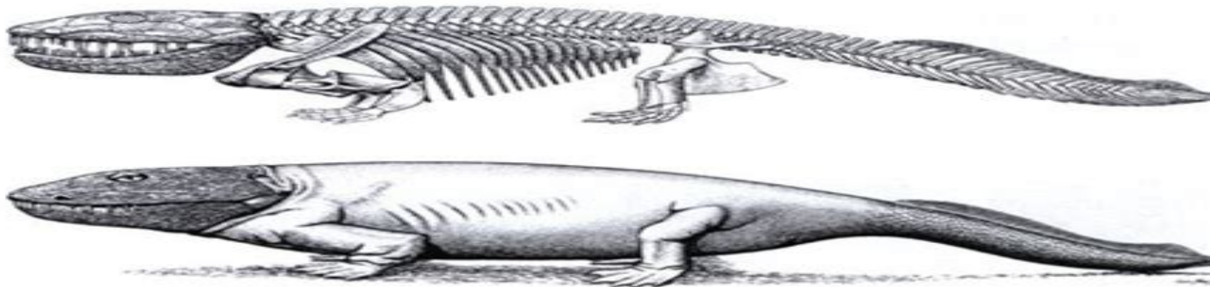
5.2. Jarvik's (1996) reconstruction of Ichthyostega.
