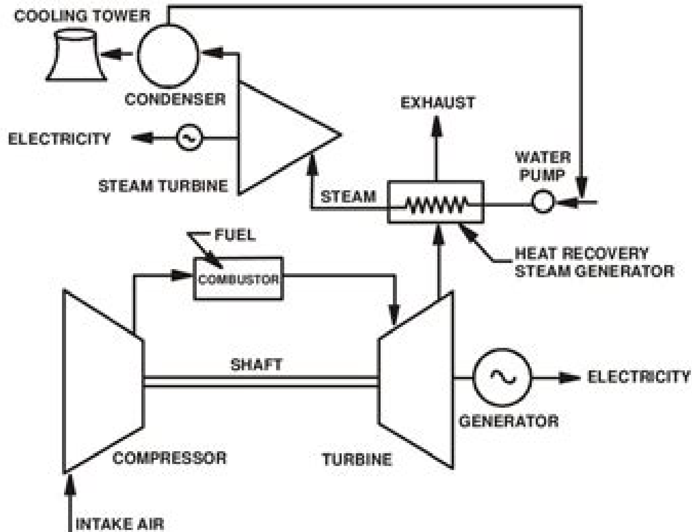
Figure 3.6c Combined-cycle power generation using natural gas
