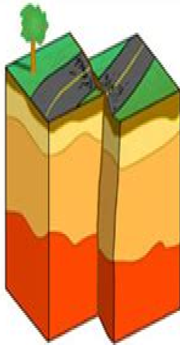
Strike-slip fault
