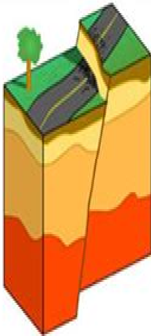
Normal fault
