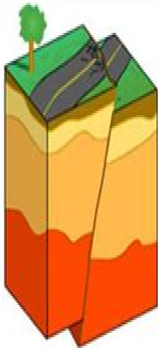
Reverse fault
