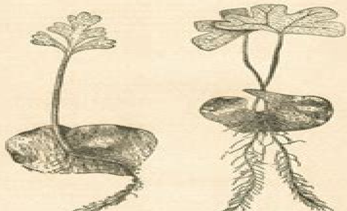
Fig. 474. Young plant of Mimosa pudica with tuberous root. Fig. 475. Transverse section of the tuberous root showing the production of a young plantlet.
