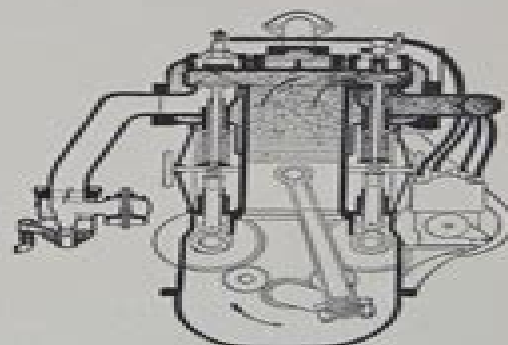
EXHAUST STROKE
