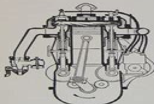
WORKING STROKE
