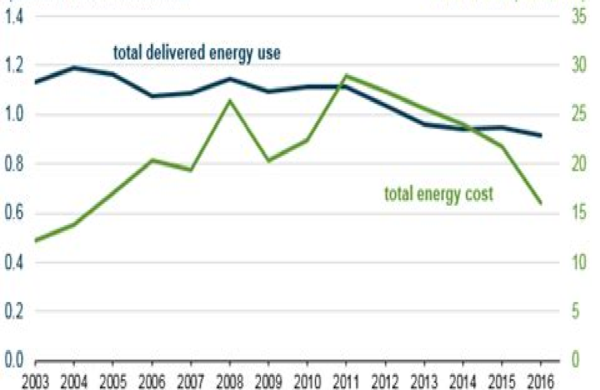
U.S. federal government energy consumption and energy cost (fiscal years 2003 - 2016) quadrillion British thermal units billion dollars (real 2016$)
