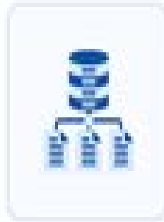
Document-oriented databases
