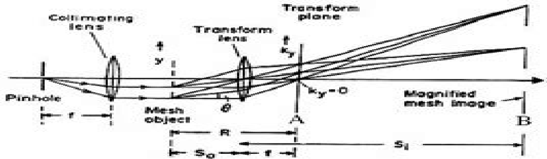
Figure 1.1: Magnified image formation with parallel coherent incident radiation.
