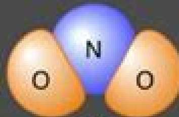
\text{NO}_2 nitrogen dioxide
