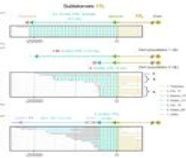
Subchromosome 10L
